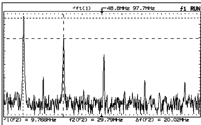
FFT measurement with the 54657A or 54659B Measurement Storage module
